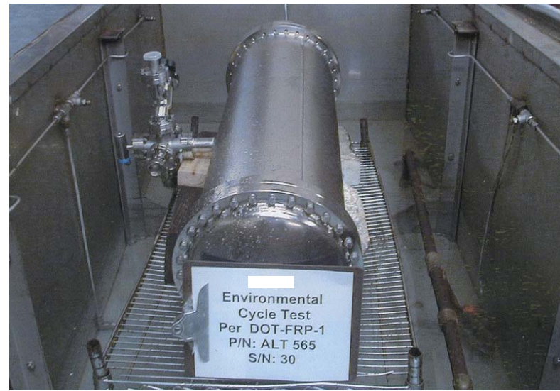
Cycle test
